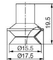
[ Rubber part ]
